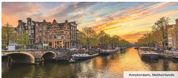
Amsterdam, Netherlands
